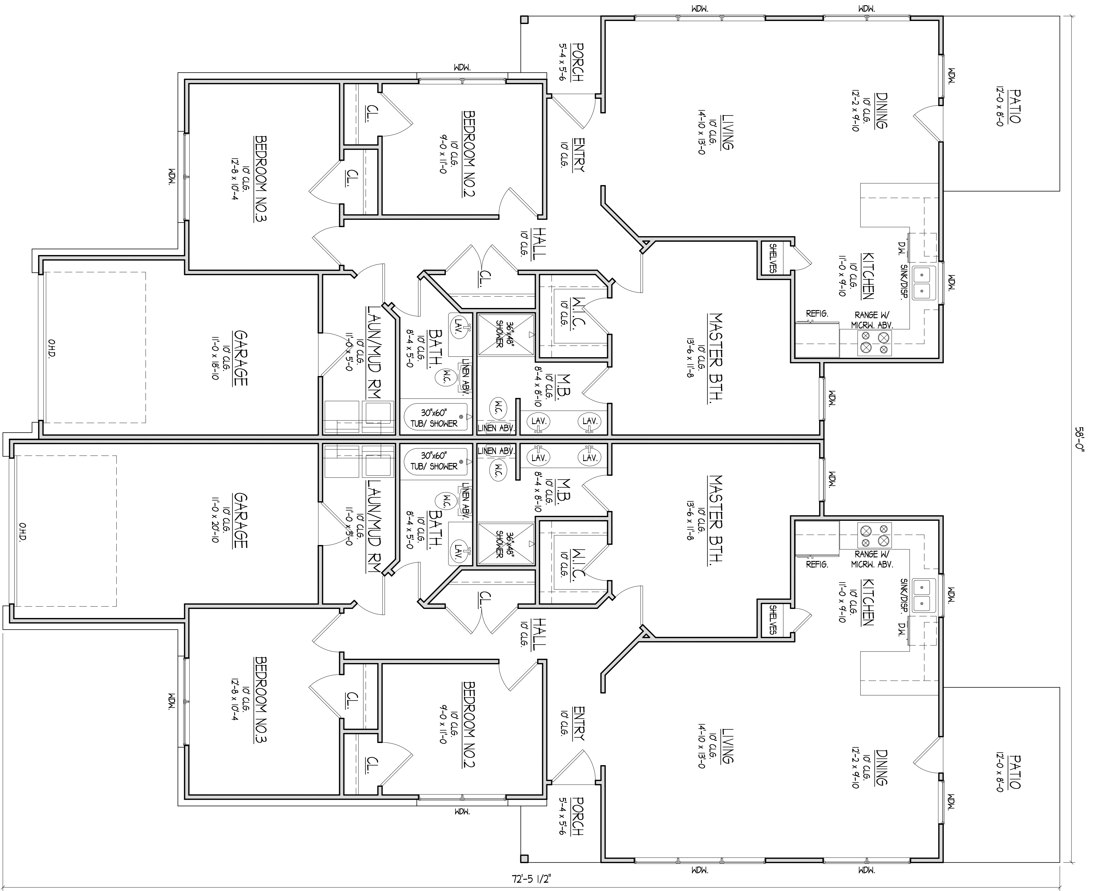
FLOOR PLAN
