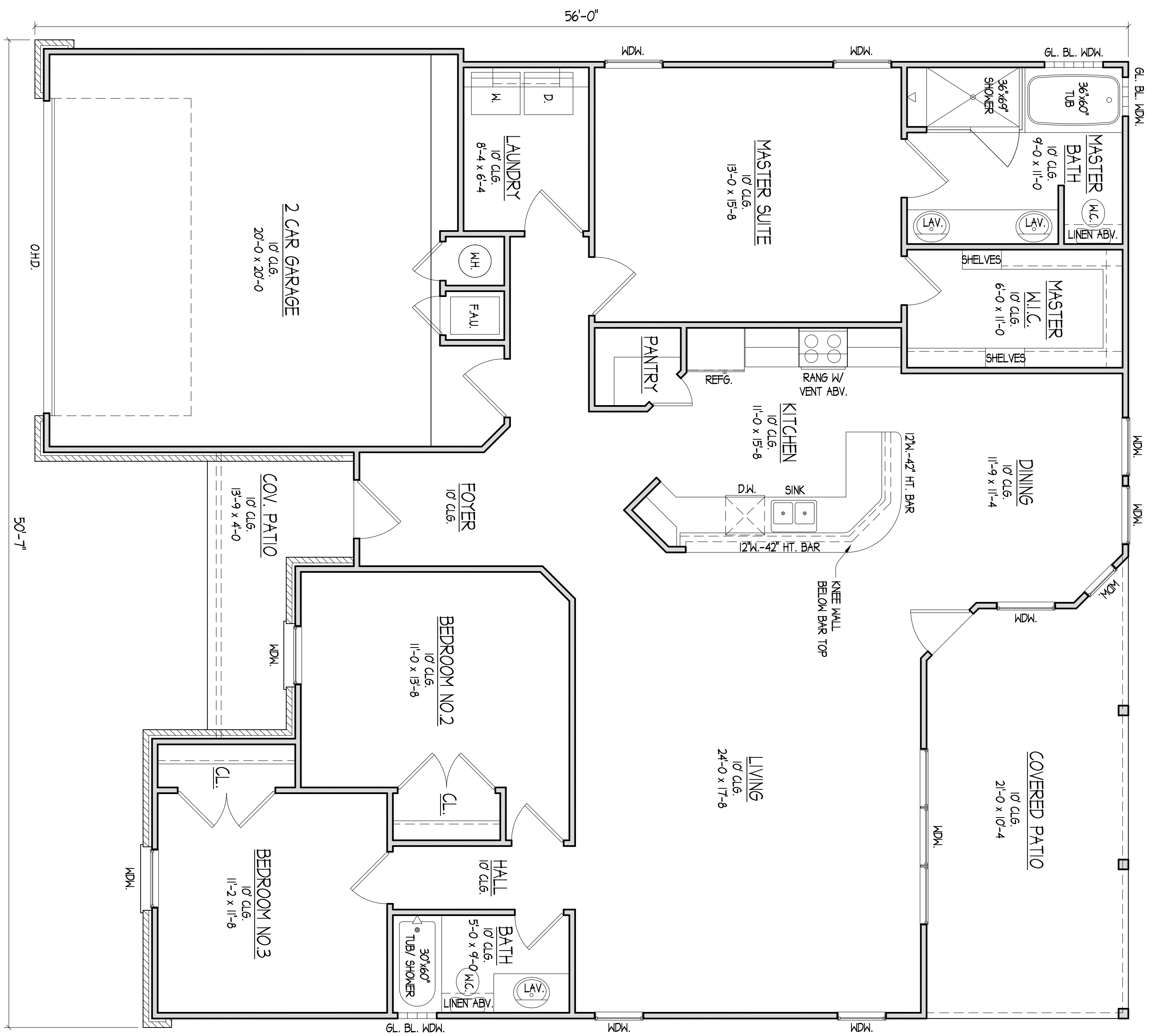
FLOOR PLAN
