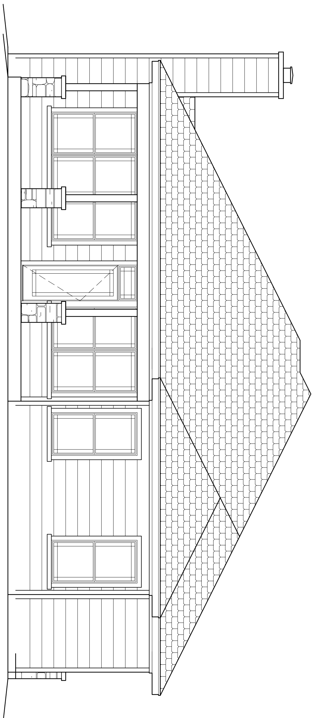
BACK ELEVATION
