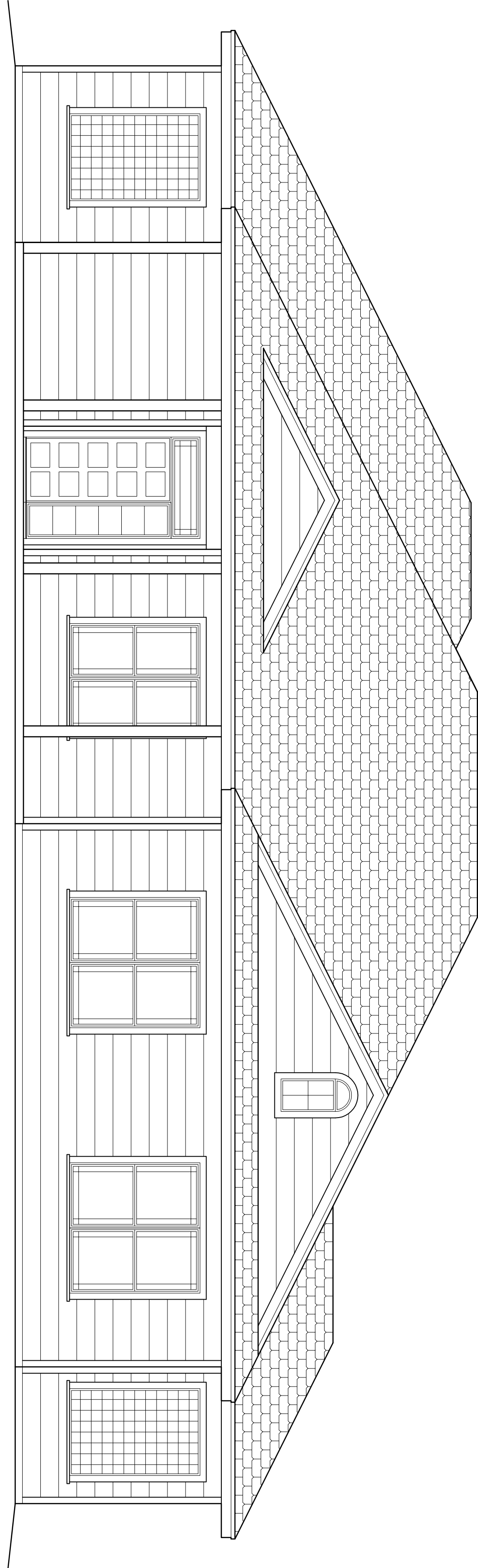
FRONT ELEVATION
