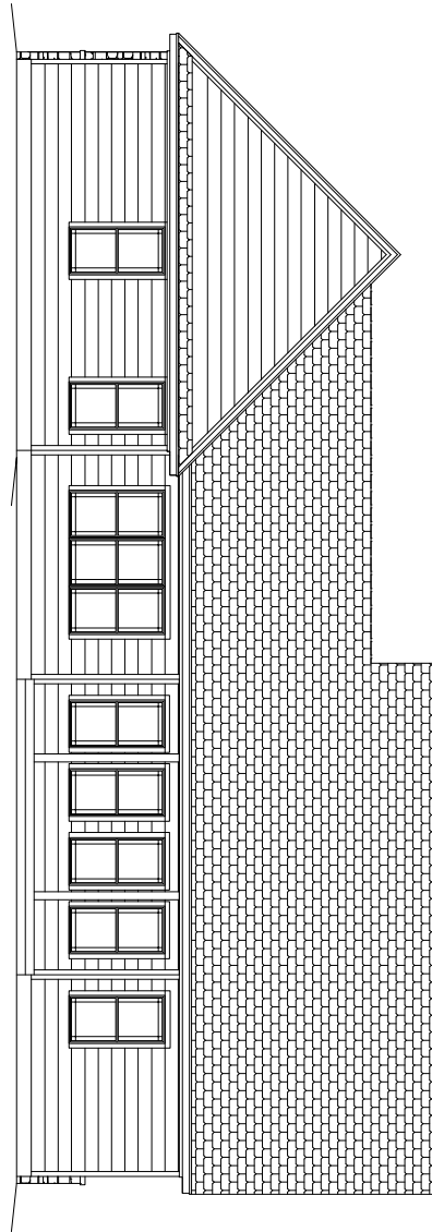
BACK ELEVATION
