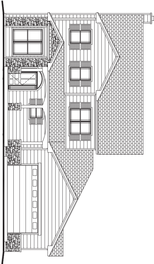
FRONT ELEVATION
